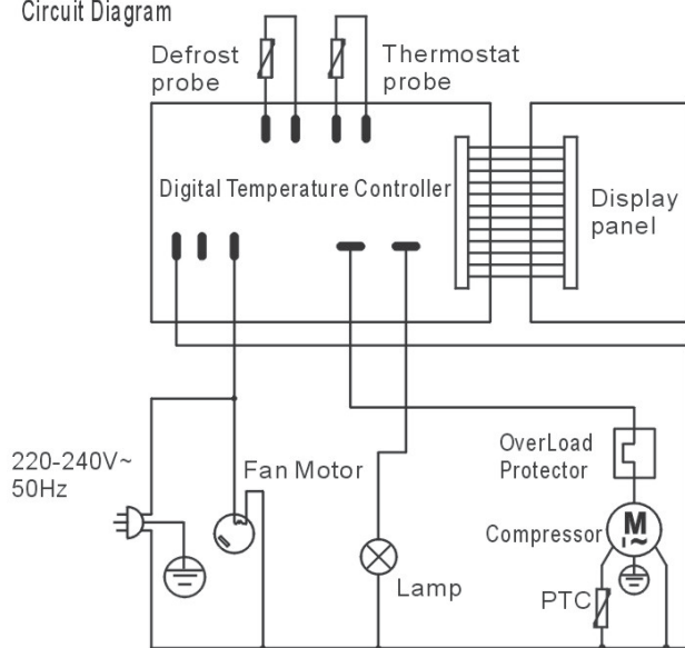
Circuit Diagram
