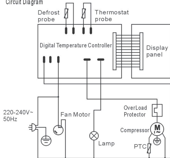
Circuit Diagram
